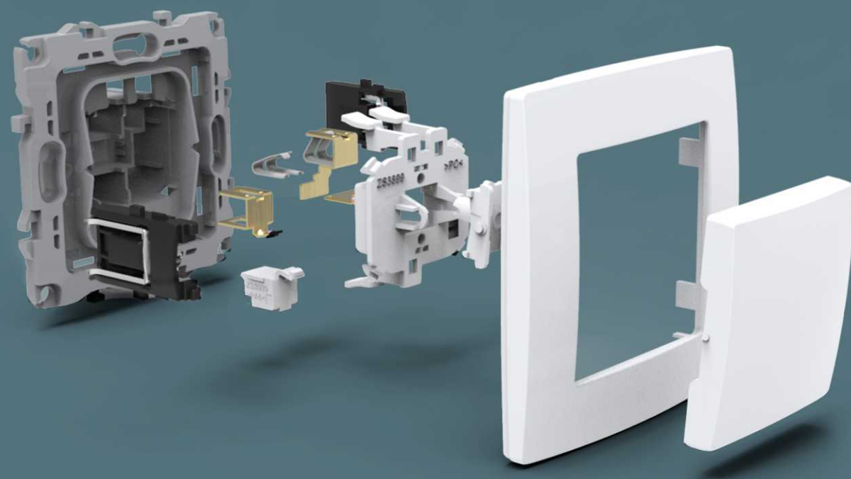
(Switch breakdown diagram)
